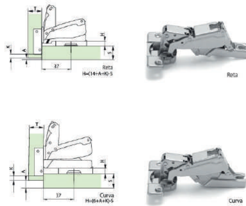
Dobradiça 175°
